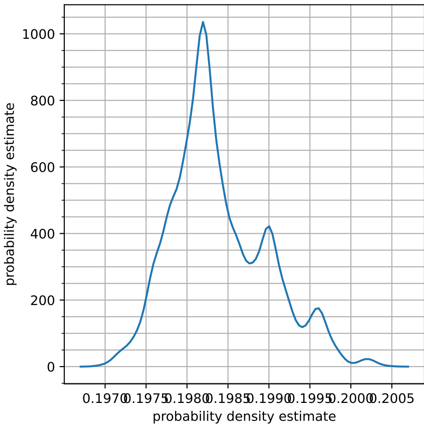
Float multiply mean= 0.198 \mu s
