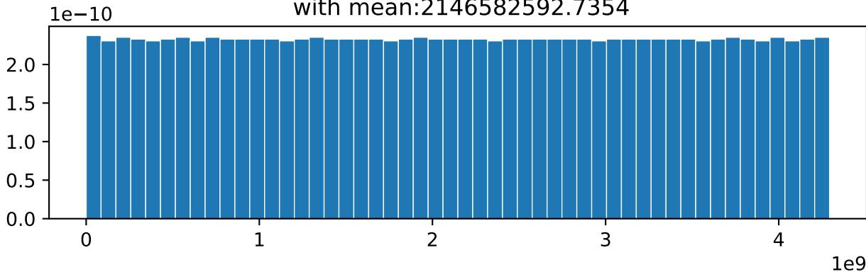
Histogram of Halton Sequence with mean:2146582592.7354
