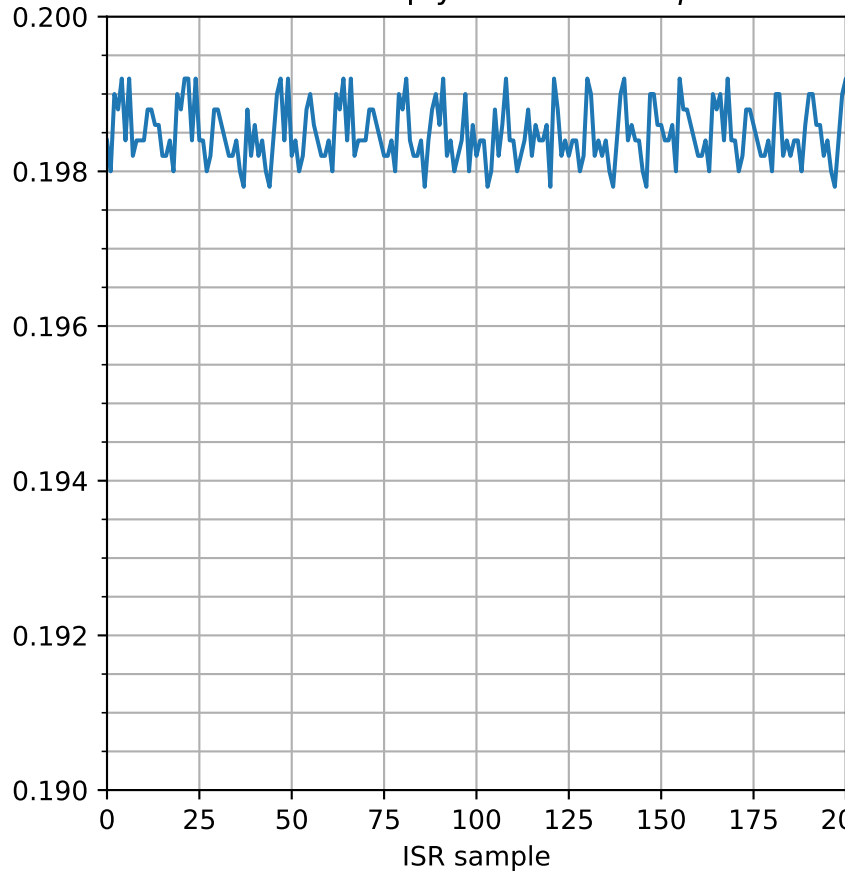
Float multiply mean= 0.198\ \mu s
